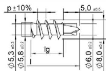
ASSY plus 3,0
