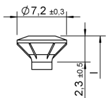
FBS-Kopf
