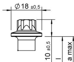
Hexalobular head with or without collar
