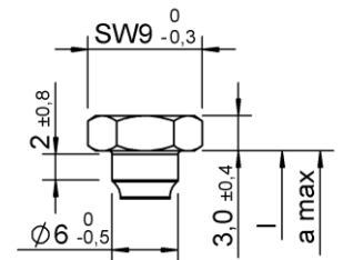
Kombi hexagonal head with and without collar
