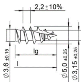
cut
