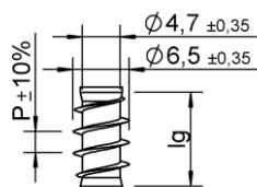
Underhead thread Lg2 < 4 x d, P = 2.6
