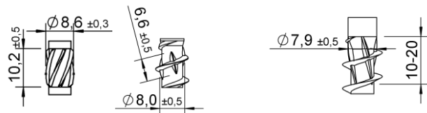
Shank cutters
