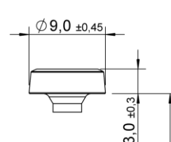
Elmo head
