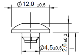
Truss head – design with and without cutter ribs and with and without flange
