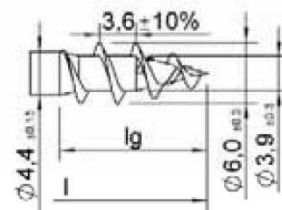
ASSY filetage large
