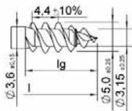
ASSY double filetage
