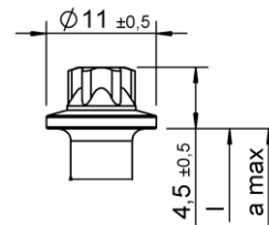
Hexalobular head with and without collar
