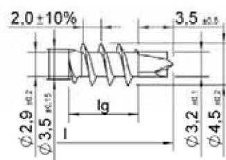
ASSY plus 3,0
