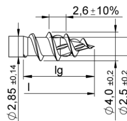
Grobgang II
