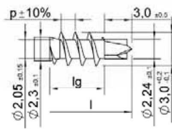
ASSY plus 3,0
