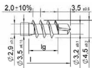
ASSY plus
