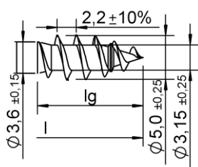
single – threaded
