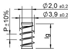
Underhead thread Lg2 < 4 \times d , P = 1.6, 2.0, 2.2, 3.2
