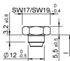
Kombi hexagonal head
