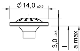
Large washer head I
