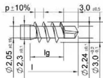
ASSY plus
