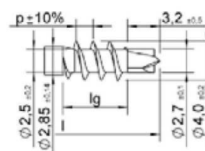
ASSY plus 3,0
