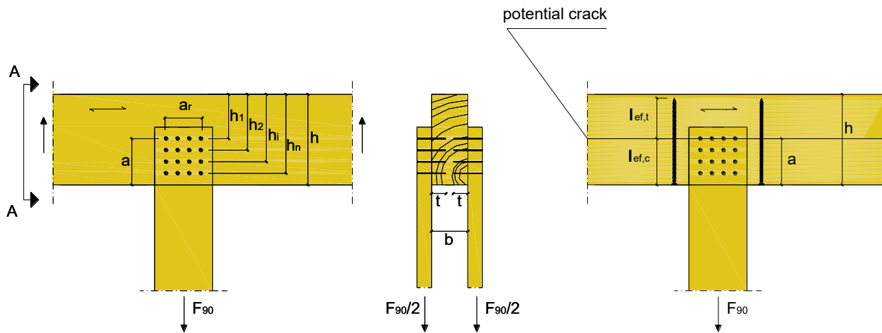
Figure A.4.1: Example for tensile reinforcement of a connection force perpendicular to the grain
