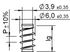
Underhead thread Lg2 < 4 x d, P = 2.6, 3.6, 5.2
