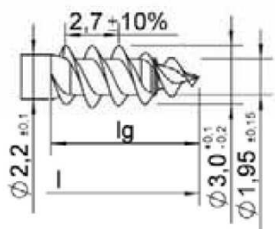
ASSY double filetage
