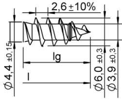
single – threaded
