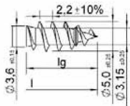
ASSY simple filetage
